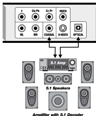
Amplifier with 5.1 Decoder
